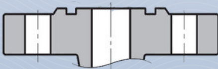
TYPE C AND D - TONGUE AND GROOVE FACE
